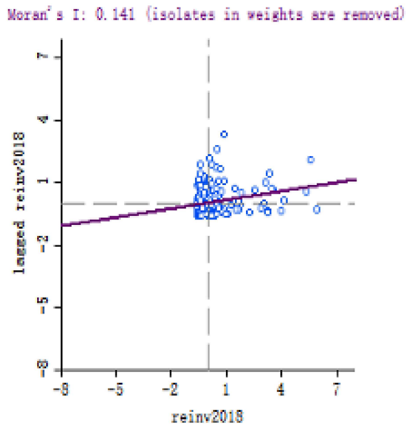
Figure 4: Moran's I for real estate investment in 2018
