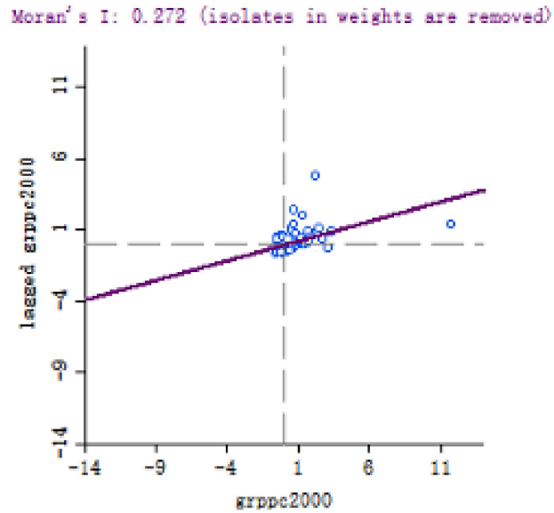
Figure 1: Moran's I for GRP per capita in 2000
