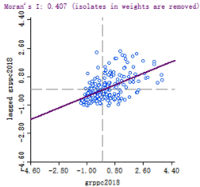
Figure 2: Moran's I for GRP per capita in 2018
